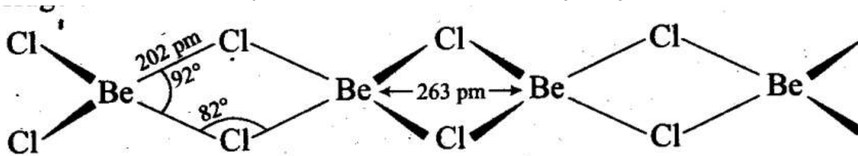
Structure of \text{BeCl}_2 in solid state
