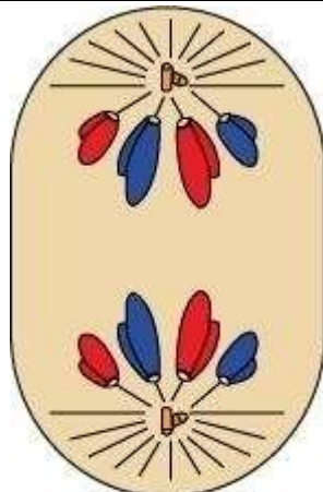
Anaphase
