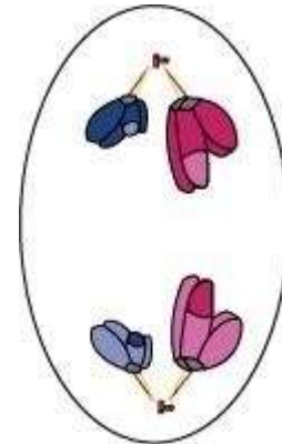
Anaphase
